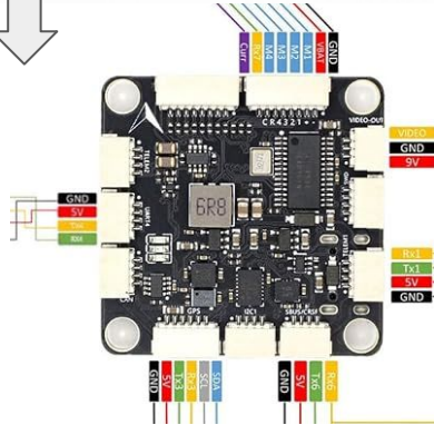
Flight Controller
